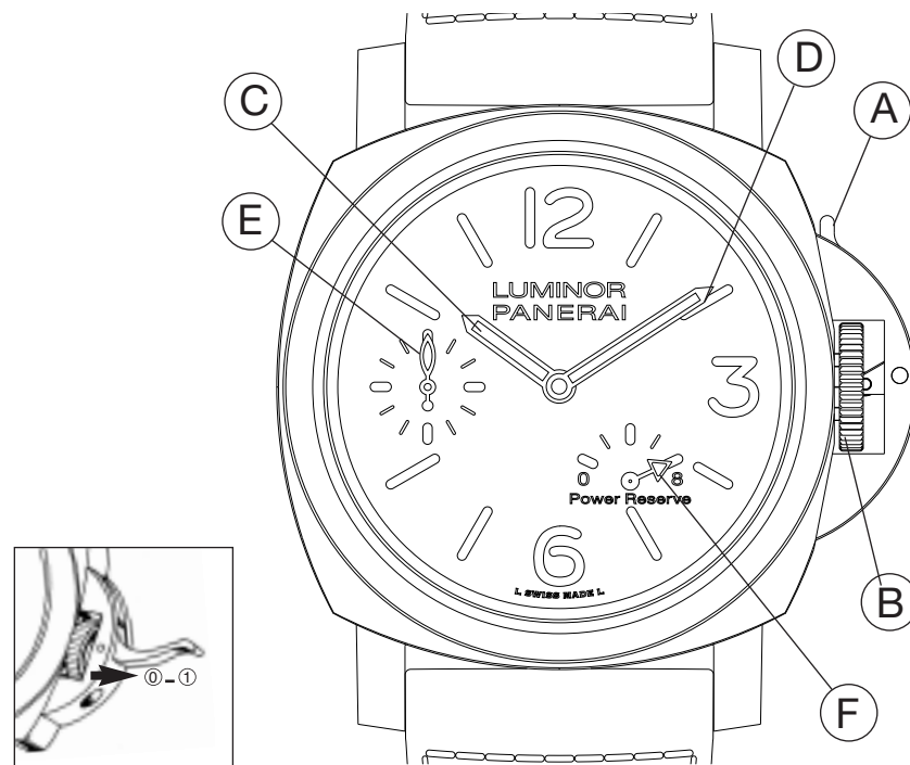
(A) LEVER (B) WINDING CROWN (C) HOURS (D) MINUTES (E) SMALL SECONDS* (F) POWER RESERVE INDICATOR*
